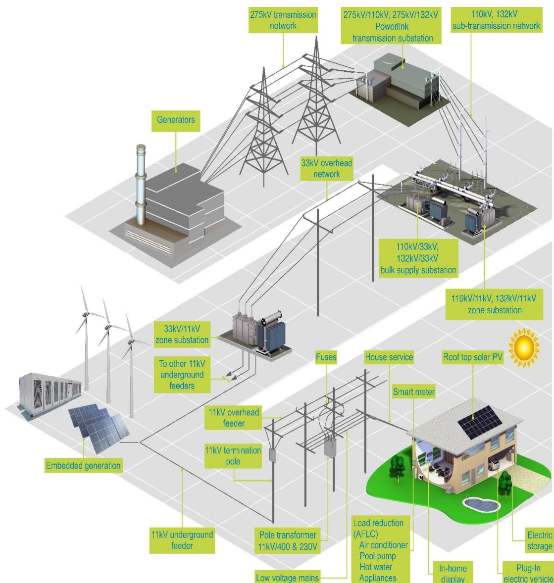
Figure 1-1 – Typical Electricity Supply Chain
