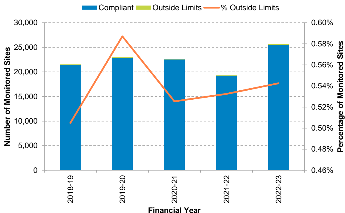
Figure 10-9 – Number of Monitored Sites Reporting Total Harmonic Distortion
