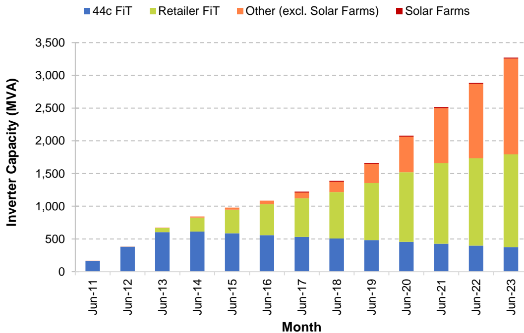
Figure 11-1 – Grid Connected solar PV System Capacity by Tariff as at June 2023
