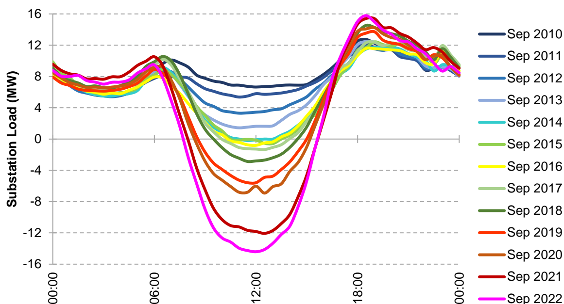
Figure 11-2 – Spring Load Profile with increasing Solar PV of North Maclean Zone Substation
