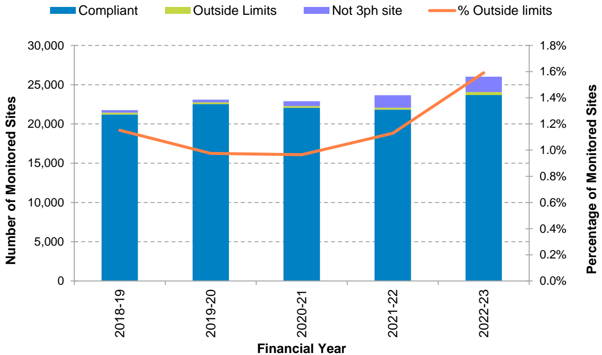
Figure 10-8 – Number of Monitored Sites Reporting Voltage Unbalance
