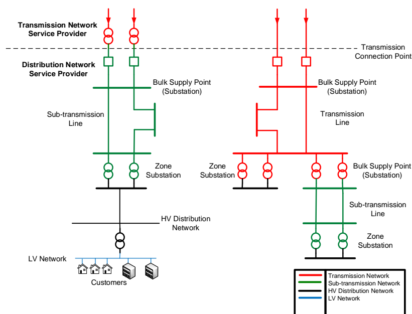
Figure 5-1 – Traditional Simplified DNSP Network
