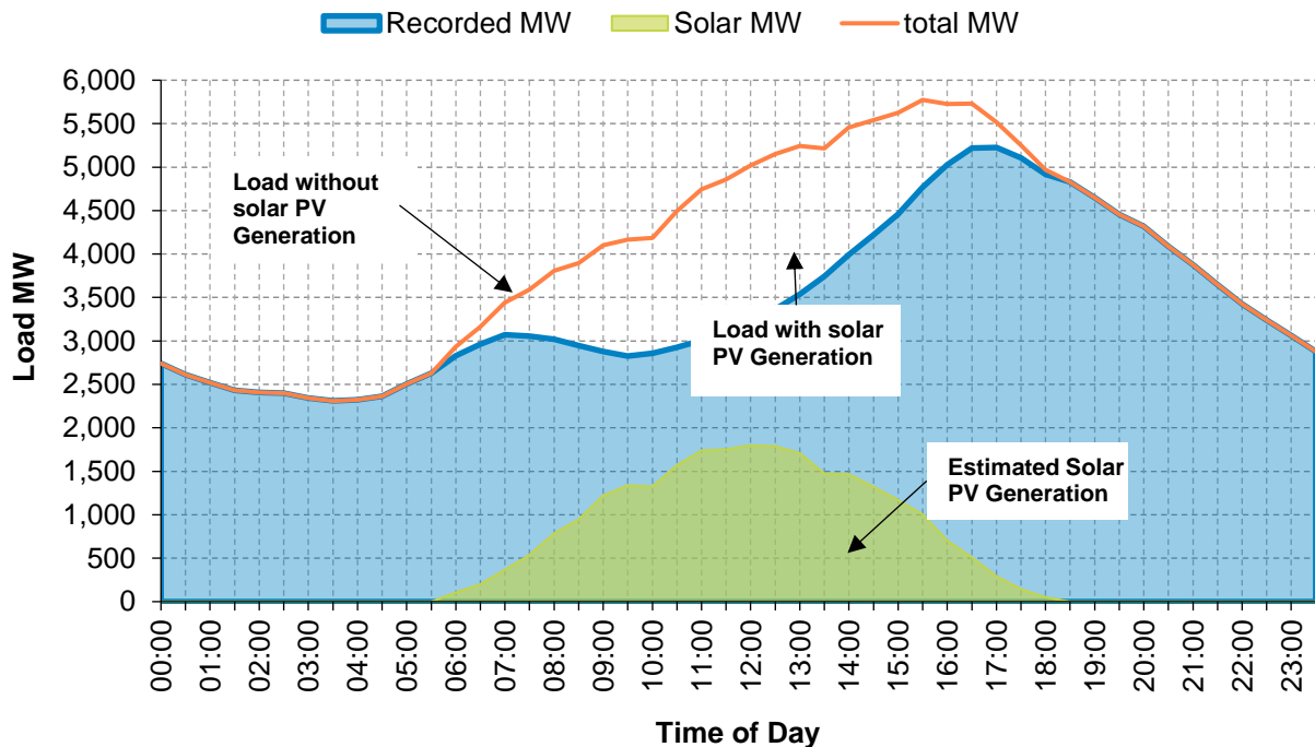
Figure 4-1 – System Demand – Solar PV Impact, 17 March 2023
