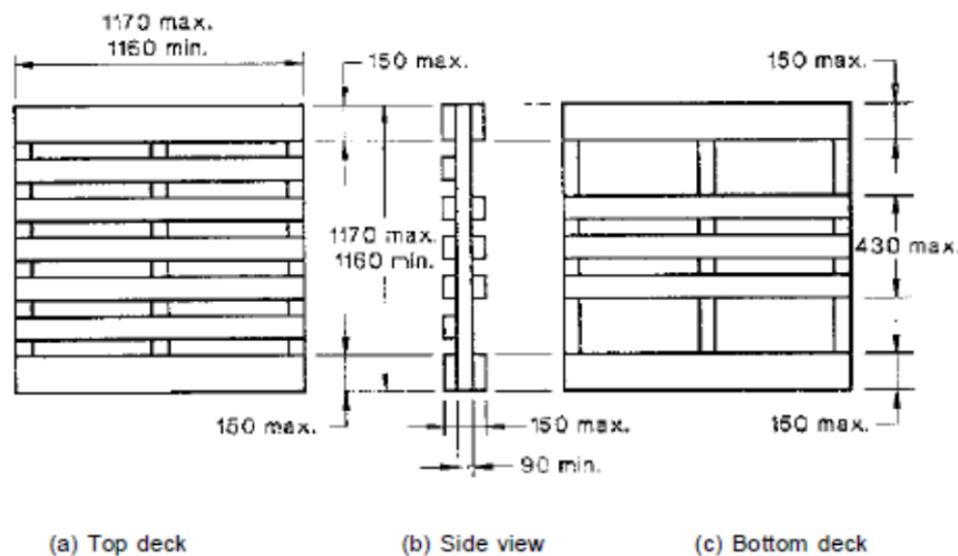
Figure A2 Timber Pallet for use in Australian Pooling Systems
