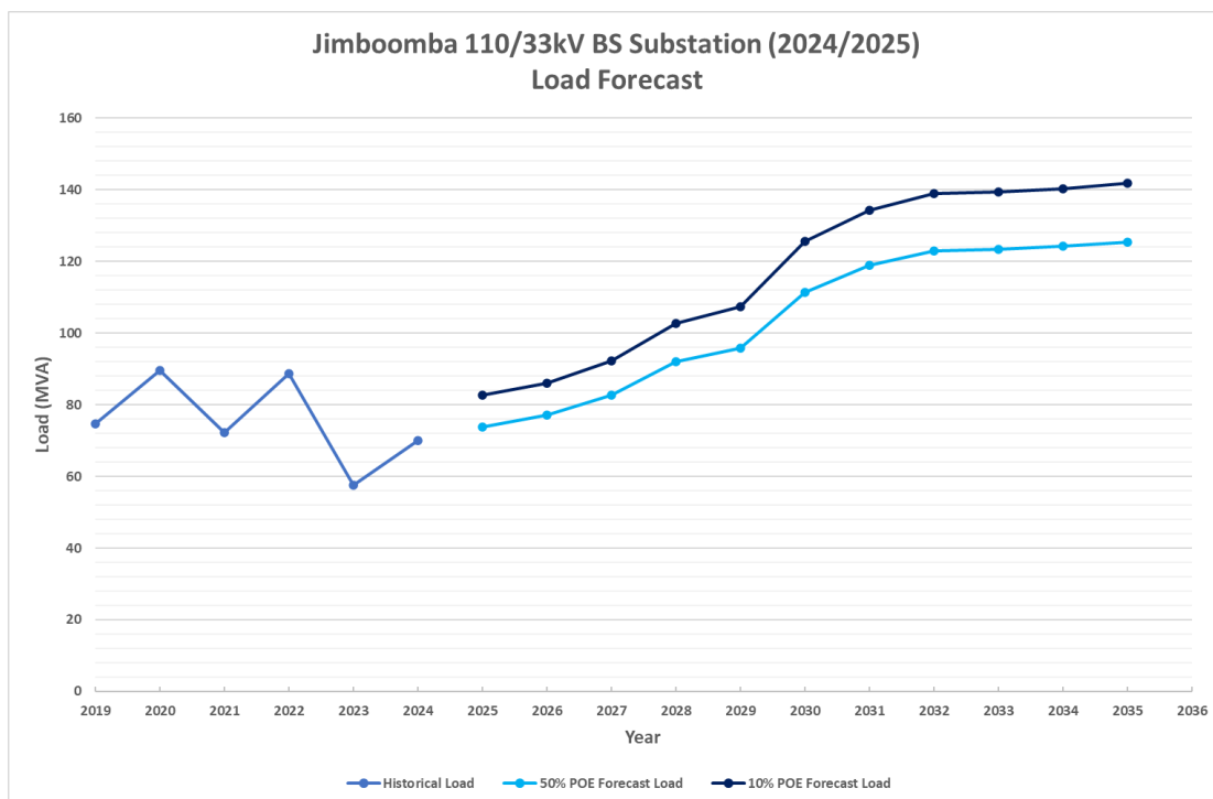
Figure 5: Jimboomba Bulk Supply Substation load forecast
