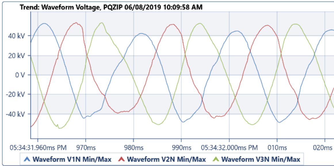
Figure 16: Measured Instantaneous Line to Neutral Voltages
